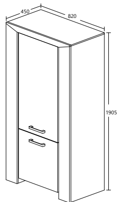
ELVIS MODEL : TW 17016-TP-S5V ITEM : TP TOWER WITH WOODEN DOOR L 82 X D 45 X H190.5cm
