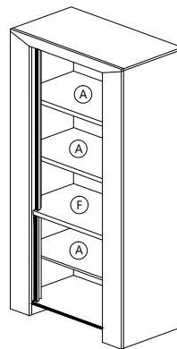
ELVIS MODEL : TW 17016-TP-S5V ITEM : TP TOWER WITH WOODEN DOOR L 82 X D 45 X H190.5cm
