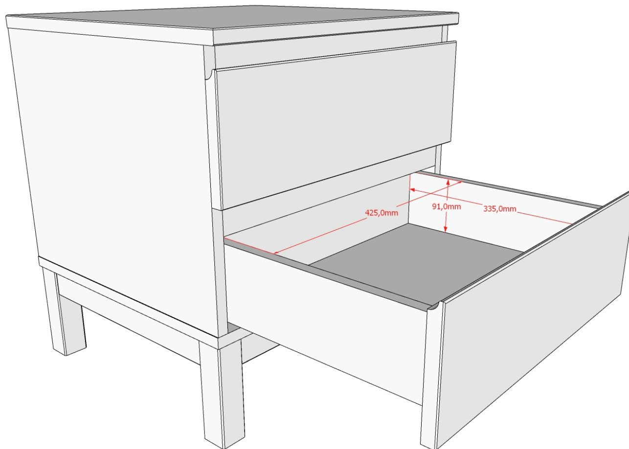
DRAWERS WITH SOFTCLOSING GLIDERS
