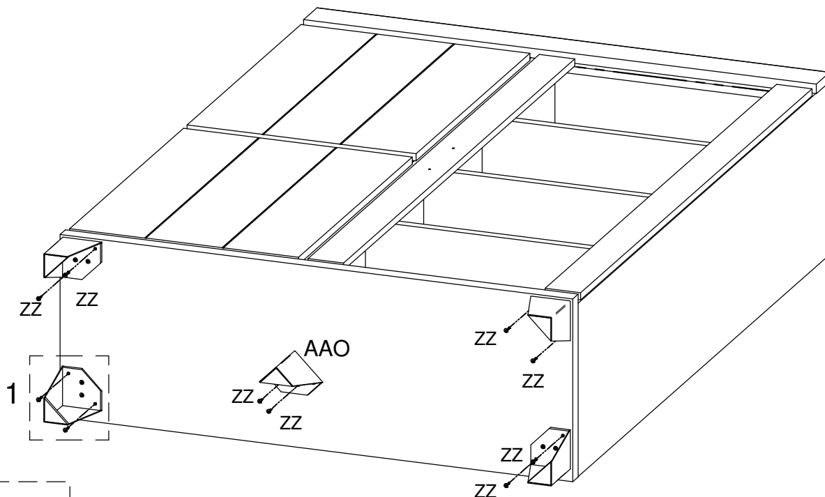
DETAIL 1
