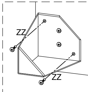
DETAIL 1
