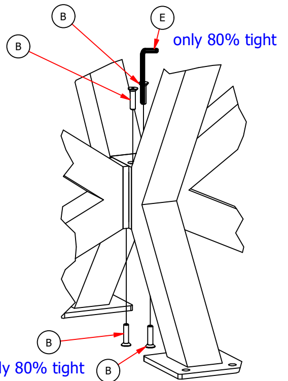
DETAIL c
