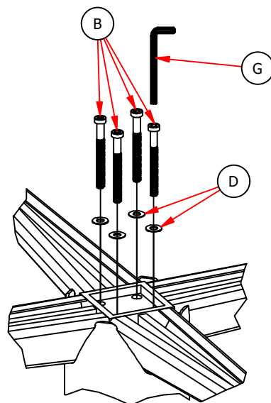
DETAIL c
