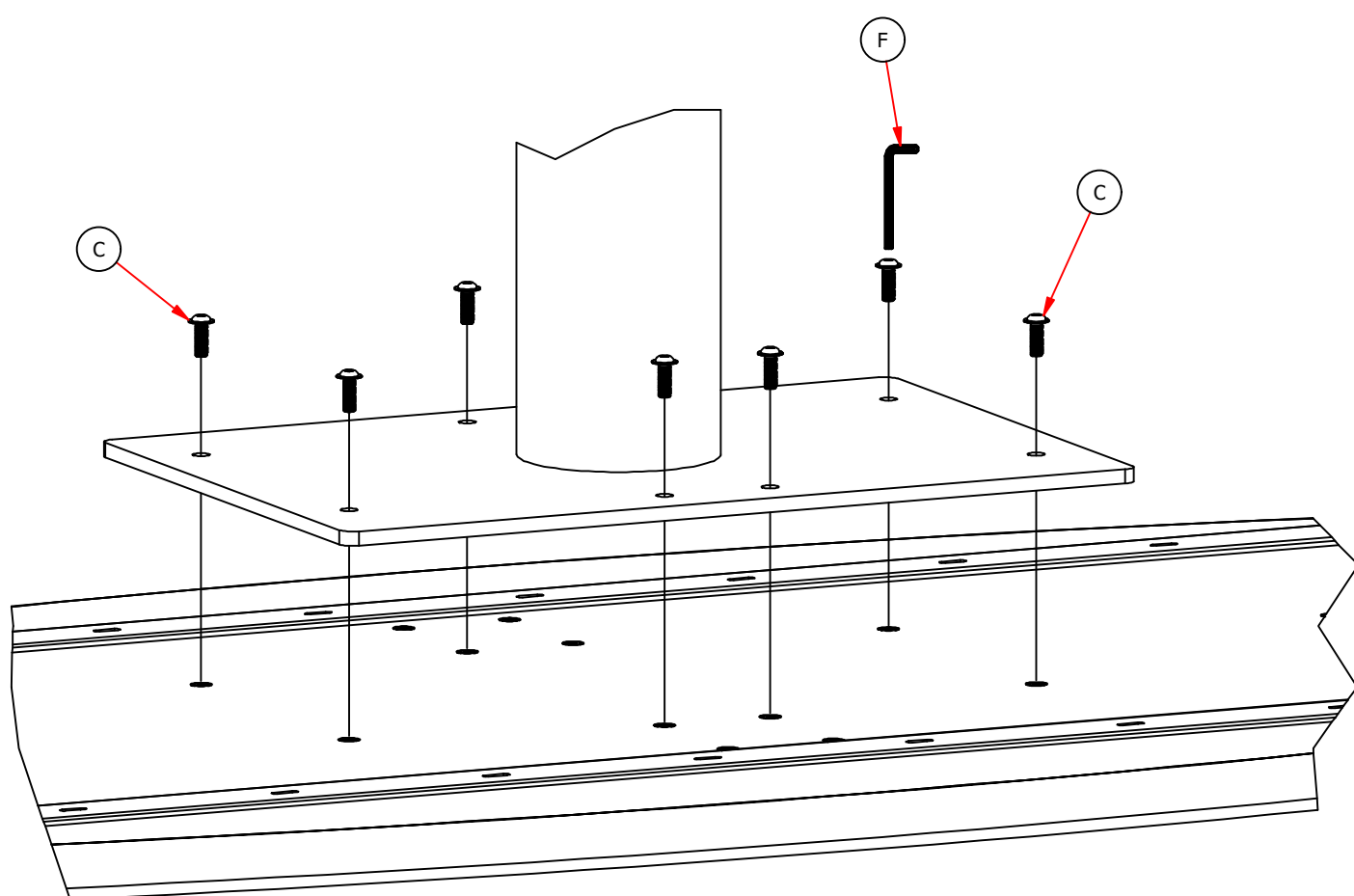
DETAIL e
