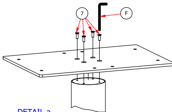
DETAIL a
