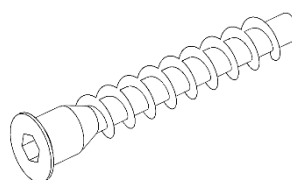
4 x Ø7x50
