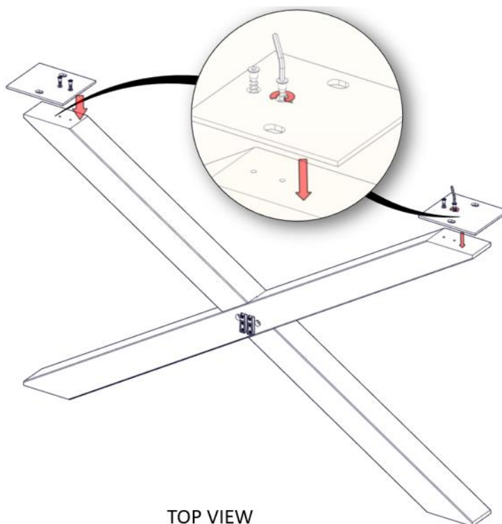
2x Rectangular plate for X profile
