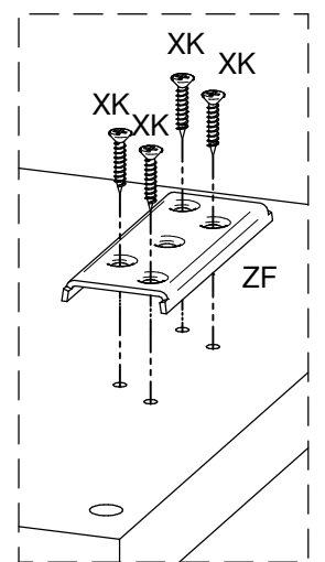
DETAIL 1
