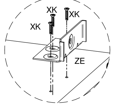
DETAIL 2
