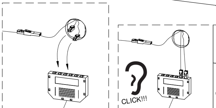
DETAIL 1
