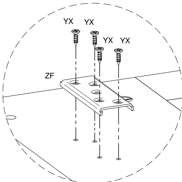
DETAIL 1
