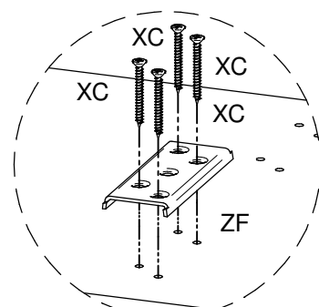
DETAIL 1
