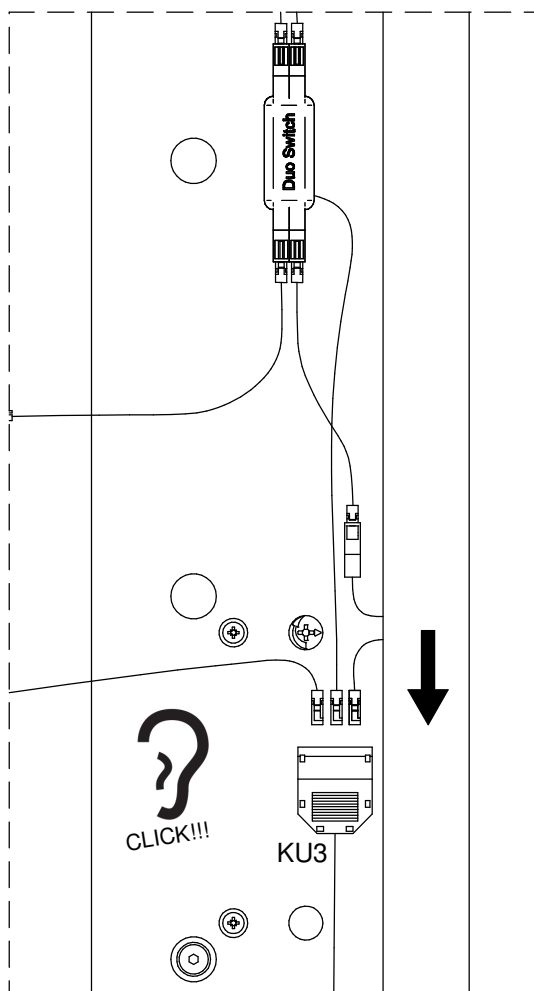
DETAIL 1
