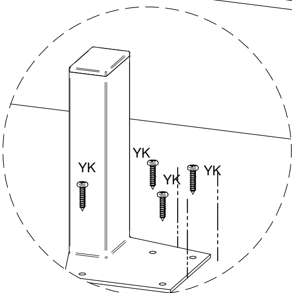
DETAIL 1
