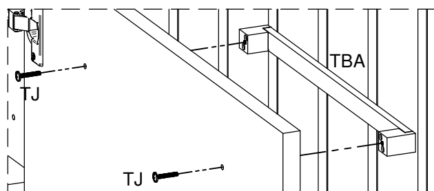
DETAIL 1
