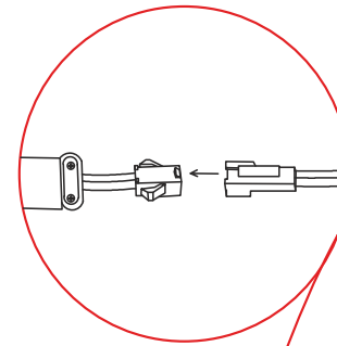
DETAIL-I
