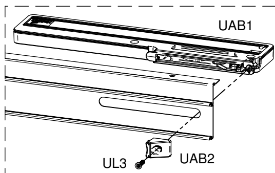
DETAIL 1
