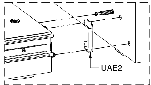
DETAIL 1
