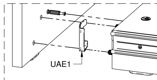
DETAIL 1
