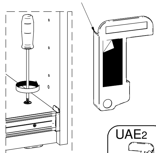
DETAIL 1
