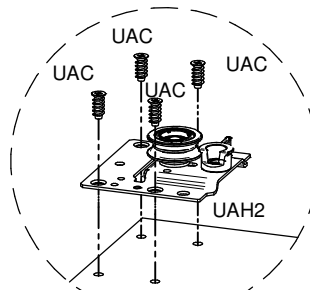
DETAIL 1
