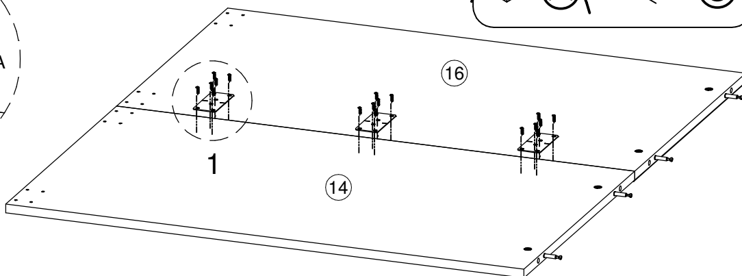
DETAIL 1
